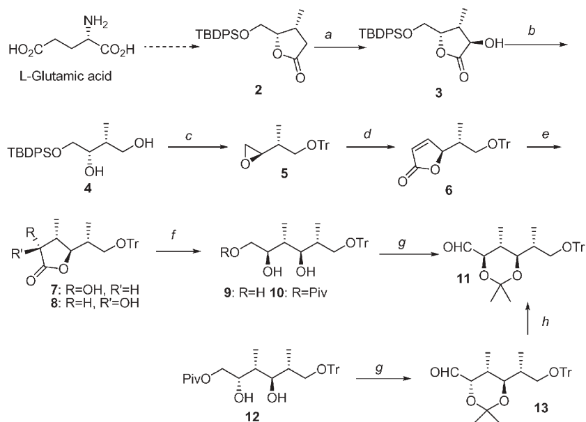
Scheme 1 a KHMDS, MoOPH, THF, -78\text{ }^{\circ}\text{C} \rightarrow -30\text{ }^{\circ}\text{C} , 78%; b 1. NaBH 4 , aq. THF; 2. NaIO 4 , aq. MeOH; then NaBH 4 ; c 1. TrCl, Et 3 N, DMAP, CH 2 Cl 2 ; 2. MsCl, Et 3 N, CH 2 Cl 2 , then n -Bu 4 NF, THF; d 1. PhSeCH 2 CO 2 H, BuLi; 2. EDAC·HCl, DMAP; 3. 30% H 2 O 2 , CH 2 Cl 2 ; e 1. CuI, MeLi·LiBr, ether, -20\text{ }^{\circ}\text{C} ; 2. KHMDS, THF, -78\text{ }^{\circ}\text{C} \rightarrow -30\text{ }^{\circ}\text{C} , MoOPH; f 1. LiAlH 4 , THF; 2. pivaloyl chloride, pyridine; g 1. camphorsulfonic acid, acetone, 2,2-dimethoxypropane; 2. LiAlH 4 , THF; h oxalyl chloride, DMSO, CH 2 Cl 2 , -78\text{ }^{\circ}\text{C} \rightarrow -30\text{ }^{\circ}\text{C} ; i K 2 CO 3 , MeOH.
