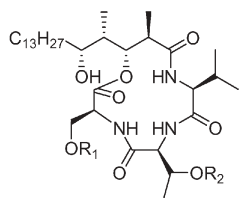
Stevastelin A3: R_1 = \text{Ac} , R_2 = \text{SO}_3\text{H} Stevastelin B3: R_1 = \text{Ac} , R_2 = \text{H} Stevastelin C3: R_1 = \text{H} , R_2 = \text{H}
