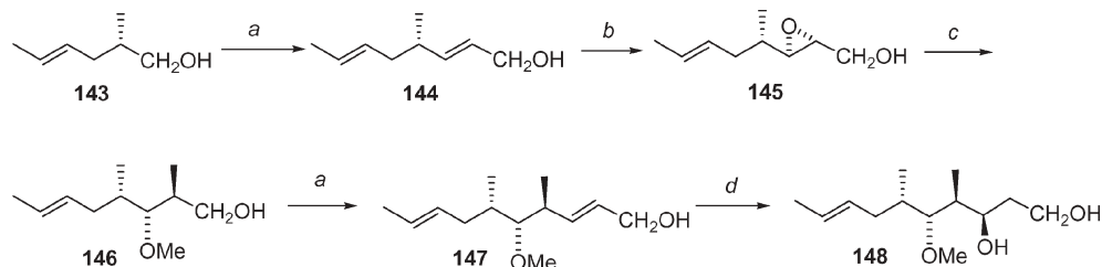
Scheme 18 a 1. IBX, DMSO, rt, 30 min; 2. \text{Ph}_3\text{CCHCO}_2\text{Et} , benzene, rt, 3 h; 3. DIBAL-H, \text{CH}_2\text{Cl}_2 , -20^\circ\text{C} , 30 min; b TBHP, \text{Ti}(\text{O}i\text{Pr})_4 , (–)-DIPT, \text{CH}_2\text{Cl}_2 , -20^\circ\text{C} , 20 h; c 1. \text{Me}_2\text{CuLi} , \text{Et}_2\text{O} , -78^\circ\text{C} , 8 h; 2. TBSCl, imidazole, \text{CH}_2\text{Cl}_2 , rt, 3 h; 3. KH, MeI, \text{Et}_2\text{O} , rt, 30 min; 4. \text{Bu}_4\text{NF} , THF, rt, 2 h; d 1. TBHP, \text{Ti}(\text{O}i\text{Pr})_4 , (+)-DIPT, \text{CH}_2\text{Cl}_2 , -20^\circ\text{C} , 18 h; 2. Red-Al, THF, 0^\circ\text{C} , 4 h.
