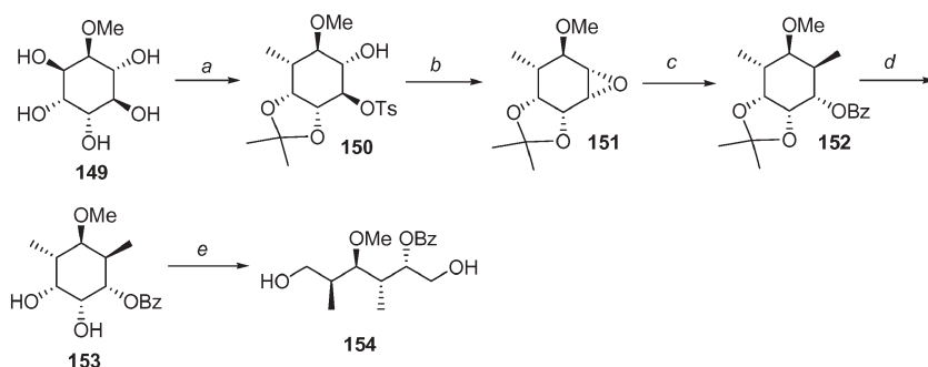
Scheme 19 a 1. ref. 36; 2. \text{Bu}_2\text{SnO} , MeOH, reflux, then TsCl, DMAP; 3. 1,4-dioxane, rt; b \text{MeONa} , MeOH, reflux; c 1. \text{Me}_3\text{Al} , \text{CH}_2\text{Cl}_2 : hexanes, rt; 2. BzCl, pyridine, DMAP, rt; d 10-camphorsulfonic acid, MeOH, rt; e \text{NaIO}_4 , acetone– \text{H}_2\text{O} , 0^\circ\text{C} , then \text{NaBH}_4 , MeOH, 0^\circ\text{C} .
