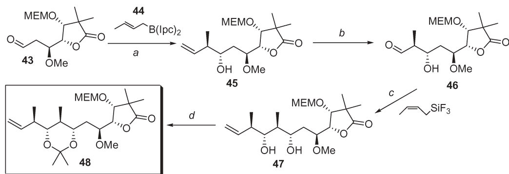
Scheme 5 a the crotyl reagent was prepared from (+)-IpcBOMe and trans -butene in THF at -78\text{ }^{\circ}\text{C} , then \text{BF}_3\cdot\text{OEt} , the aldehyde 43 , -78\text{ }^{\circ}\text{C} , 1 h, then ethanolamine; b \text{O}_3 , \text{CH}_2\text{Cl}_2 , -78\text{ }^{\circ}\text{C} , then triphenylphosphine, rt, 3 h; c aldehyde 46 , 4 Å MS, \text{CH}_2\text{Cl}_2 , rt, 0.5 h, then 0\text{ }^{\circ}\text{C} , DIPEA, ( Z )-crotyl trifluorosilane, 4 h; d 2-methoxy propene, pyridinium p -toluenesulfonate (PPTS) (cat.), \text{CH}_2\text{Cl}_2 , rt, 0.5 h.
