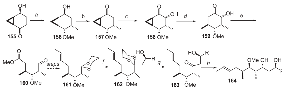
Scheme 20 a 1. DHP, PPTS, CH 2 Cl 2 , rt; 2. LDA, HMPA, THF, −78 °C, then MeI; 3. L-Selectride, THF, −78 °C; 4. NaH, MeI, TBAI, THF, 60 °C; 5. aq. HCl, MeOH, 0 °C; b Dess–Martin oxidation; c 1. TBSOTf, Et 3 N, CH 2 Cl 2 , 0 °C; 2. cat. OsO 4 , NMO, THF, H 2 O, rt; d LHMDs, THF, −78 °C, then Li, liq. NH 3 , then NH 4 Cl; e Pb(OAc) 4 , benzene, MeOH, rt; f n -BuLi, HMPA, THF, 0 °C, then RX; g Hg(ClO 4 ) 2 , CaCO 3 , THF, H 2 O, rt; h LiAlH(O t Bu) 3 , LiI, ether, −78 °C to >0 °C.
