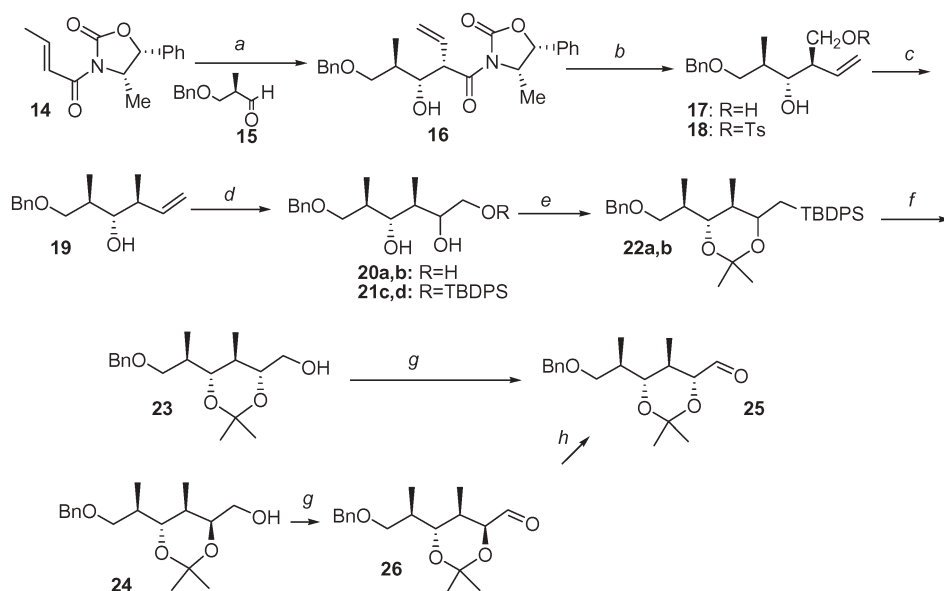
Scheme 2 a Bu 2 BOTf, Et 3 N, CH 2 Cl 2 , -78\text{ }^{\circ}\text{C} , 15 , -78\text{ }^{\circ}\text{C} , H 2 O 2 , MeOH; b 1. Bu 3 B, HOAc, THF; 2. LiBH 4 , THF, 0\text{ }^{\circ}\text{C} ; 3. H 2 O 2 , MeOH; c 1. p -TolSO 2 Cl, pyridine, 5\text{ }^{\circ}\text{C} ; 2. Li(Et) 3 BH, THF; 3. H 2 O 2 , NaOH (aq), MeOH; d 1. OsO 4 , R 3 N·O, H 2 O/Me 2 CO; 2. TBDPSCl, Et 3 N, DMAP, CH 2 Cl 2 ; e Me 2 C(OMe) 2 , CSA, acetone; f ( n -Bu) 4 NF, THF; g Pyr·SO 3 , Et 3 N, DMSO; h K 2 CO 3 , MeOH.
