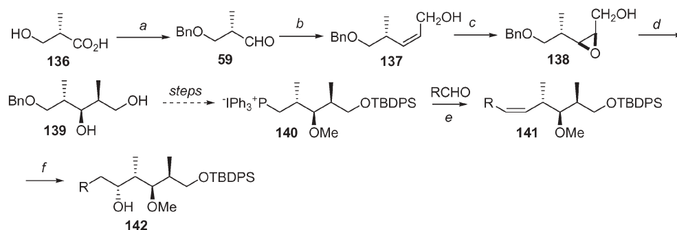
Scheme 17 a 1. \text{PhCH}_2\text{OC}(=\text{NH})\text{CCl}_3 , \text{CF}_3\text{SO}_3\text{H} ; 2. \text{LiAlH}_4 ; 3. Swern oxidation; b 1. (\text{CF}_3\text{CH}_2\text{O})_2\text{P}(=\text{O})\text{CH}_2\text{CO}_2\text{Me} , \text{KN}(\text{TMS})_2 , 18-Crown-6; 2. DIBAL-H; c MCPBA; d \text{Me}_2\text{CuLi} ; e n\text{-BuLi} ; f \text{B}_2\text{H}_6 , \text{H}_2\text{O}_2 .
