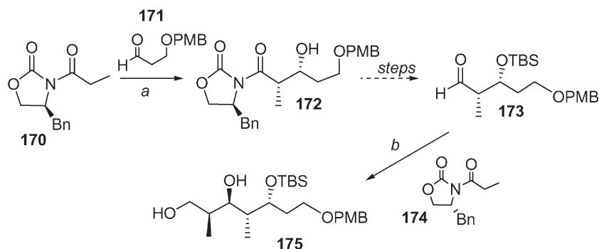
Scheme 22 a n -Bu 2 BOTf, CH 2 Cl 2 , Et 3 N, −5 °C, then −78 °C, 171; b 1. 174, n -Bu 2 BOTf, CH 2 Cl 2 , Et 3 N, −5 °C, then −78 °C, 173; 2. LiBH 4 , THF–MeOH, 0 °C.
