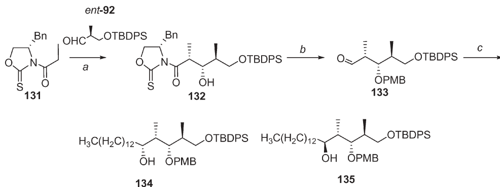
Scheme 16 a TiCl 4 , DIPEA, CH 2 Cl 2 , −78 °C; b 1. NaBH 4 , EtOH, 0 °C; 2. MeOPhCH(OMe) 2 , CSA (cat.), CH 2 Cl 2 ; 3. DIBAL-H, CH 2 Cl 2 , −78 °C to >0 °C; 4. Swern oxidation; c CH 3 (CH 2 ) 12 MgBr, THF, 0 °C to >rt.
