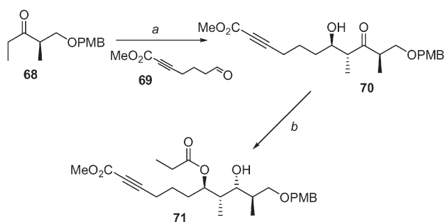
Scheme 8 a (c-Hex) 2 BCl, Et 3 N, Et 2 O, 0 °C, 1 h, then –78 °C and 69 to >–20 °C, 12 h, oxidative work-up; b SmI 2 , EtCHO, THF, 0 °C, 15 min, then 70 , 0 °C, 2 h.
