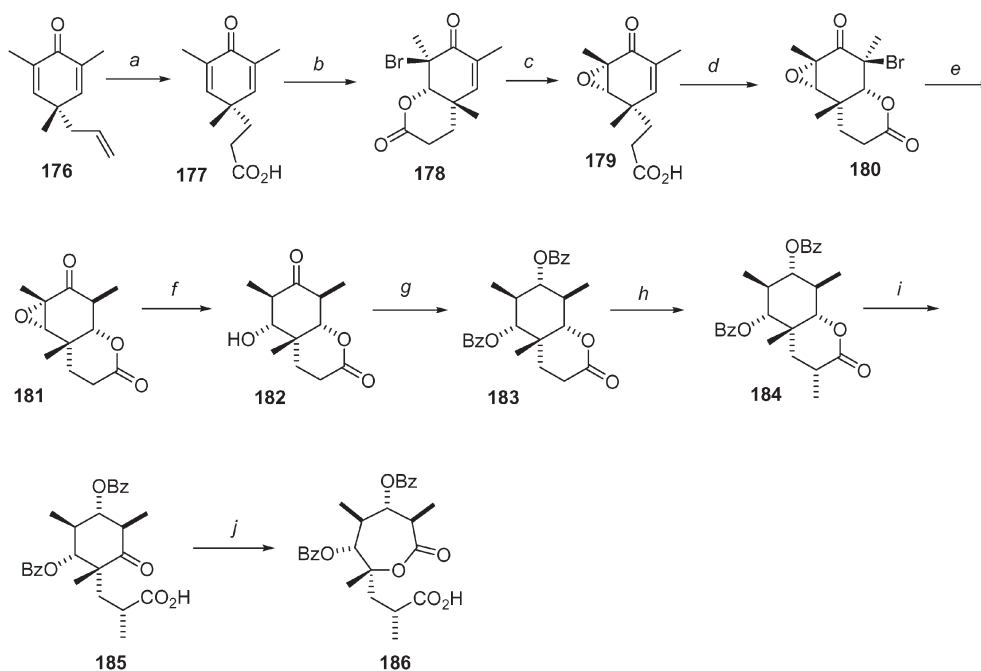
Scheme 23 a 1. \text{B}_2\text{H}_6 , THF, 0-10^\circ\text{C} ; 2. Jones chromic acid, 0-10^\circ\text{C} ; b \text{Br}_2 , KBr, \text{H}_2\text{O} ; c aq. KOH, THF; d \text{Br}_2 , KBr, \text{H}_2\text{O} ; e \text{Bu}_3\text{SnH} , AIBN, PhH; f \text{Al/Hg} , THF, \text{H}_2\text{O} , 0 to -10^\circ\text{C} ; g 1. \text{H}_2 , Raney Ni, DME, -20^\circ\text{C} ; 2. \text{BzCl} , pyridine; h LDA, THF, -78^\circ\text{C} , then MeI, HMPA, -78^\circ\text{C} to >-45^\circ\text{C} ; i 1. LiOH, \text{H}_2\text{O} ; 2. \text{CrO}_3 , \text{H}_2\text{SO}_4 , acetone, -10^\circ\text{C} ; j \text{MeCO}_3\text{H} , EtOAc, 55^\circ\text{C} .
