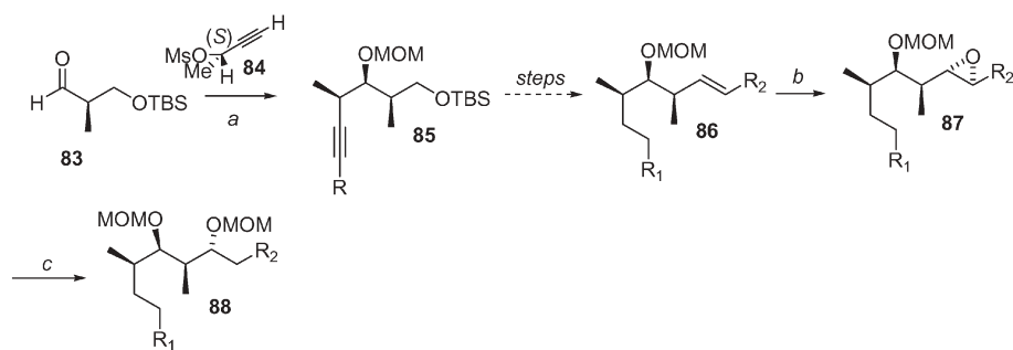
Scheme 10 a 1. Pd(dppf)Cl 2 , InI, THF–HMPA; 2. MOMCl, Bu 4 NI, i -Pr 2 NEt; b (+)-DIPT, Ti(O- i -Pr) 4 , t -BuOOH; c 1. Red-Al, THF; 2. MOMCl, Bu 4 NI, i -Pr 2 NEt.
