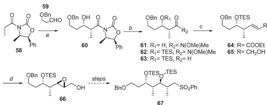
Scheme 7 a Bu 2 BOTf, Et 3 N, CH 2 Cl 2 , 0 °C, then 59 , –78 °C, 2 h to >0 °C, 2 h; b 1. Me 3 Al, MeONHMe·HCl, THF, toluene, CH 2 Cl 2 , –10 to >0 °C, 1.5 h; 2. TESCl, imidazole, DMF, 23 °C, 35 min; 3. DIBAL-H, THF, hexane, –78 °C, 2 h; c 1. ( i -PrO) 2 P(O)CH 2 COOEt, t -BuOK, THF, –78 °C, 1.5 h to >0 °C, 1.5 h; 2. DIBAL-H, CH 2 Cl 2 , hexane, –78 °C, 1.5 h; d Ti(O- i -Pr) 4 , (–)-DET, t -BuOOH, 4 Å MS, CH 2 Cl 2 , –23 °C, 2 h.
