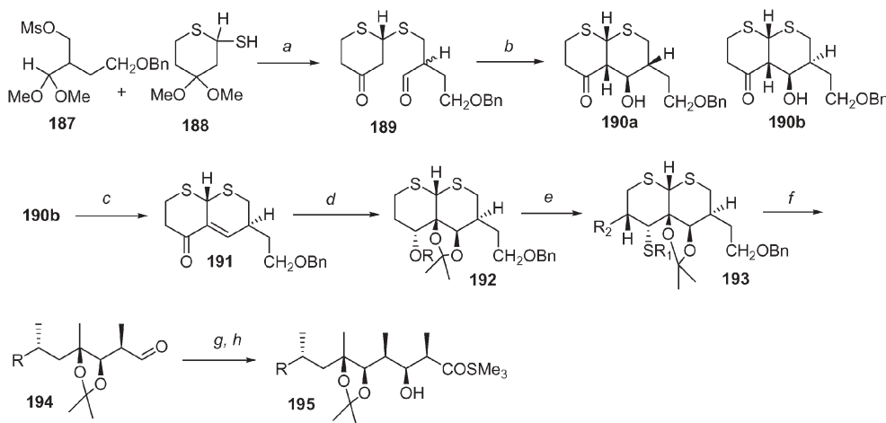
Scheme 24 a 1. NaH, THF, DMSO, rt; 2. AcOH, \text{H}_2\text{O} , rt; b D-Pro, PhH–MeOH, rt; c 1. MsCl, py; 2. \text{Al}_2\text{O}_3 , EtOAc; d 1. \text{NaBH}_4 , MeOH, 0^\circ\text{C} ; 2. \text{MeOCH}_2\text{I} , KH, THF; 3. \text{OsO}_4 , \text{Et}_2\text{O} , then \text{NaHSO}_3 , py; 4. \text{Me}_2\text{C}(\text{OMe})_2 , TsOH, \text{CH}_2\text{Cl}_2 ; e six steps; f 1. Raney Ni (W2), EtOH, DMF, rfx; 2. o\text{-NO}_2\text{PhSeCN} , n\text{Bu}_3\text{P} , THF, 30% \text{H}_2\text{O}_2 , THF, rt; 3. \text{O}_3 , MeOH, \text{CH}_2\text{Cl}_2 , -78^\circ\text{C} , then \text{Me}_2\text{S} , \text{NaHCO}_3 ; g 1. \text{EtCOSMe}_3 , LDA, THF, -110^\circ\text{C} ; 2. t\text{-BuLi} , THF, -110^\circ\text{C} , then AcOH, -110^\circ\text{C} ; h 1. t\text{-BuLi} , (\text{CH}_2\text{NMe}_2)_2 , THF, -110^\circ\text{C} ; 2. AcOH, -110^\circ\text{C} .
