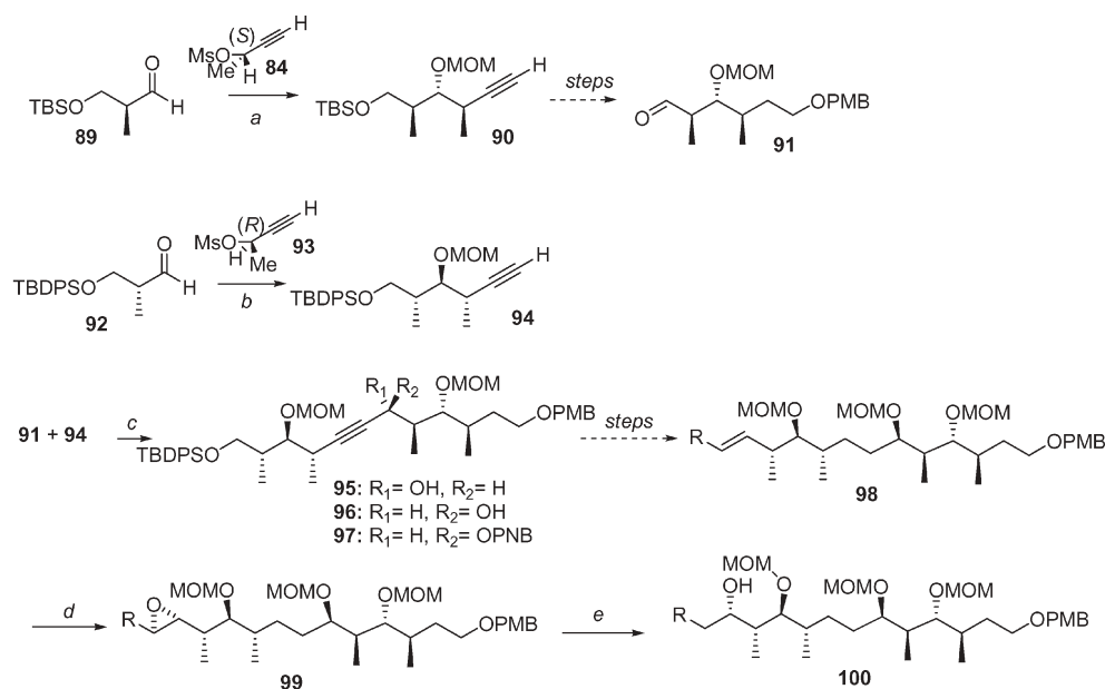
Scheme 11 a 1. Pd(dppf)Cl 2 , InI, THF–HMPA; 2. MOMCl, Bu 4 NI, i -Pr 2 NEt; b 1. Pd(dppf)Cl 2 , InI, THF–HMPA; 2. MOMCl, Bu 4 NI, i -Pr 2 NEt; c lithiation of 94 , then 91 ; d (–)-DIPT, Ti(O- i -Pr) 4 , t -BuOOH; e Zn, MeOH, Δ.
