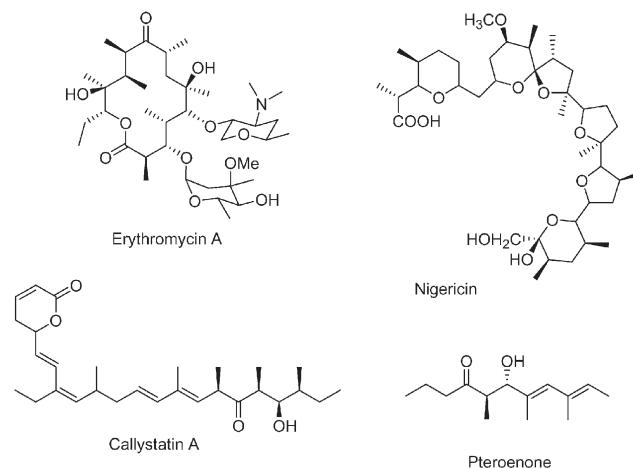
Fig. 1 Examples of naturally occurring polyketides.
