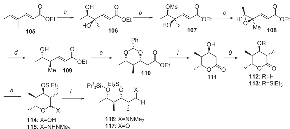
Scheme 13 a (\text{DHQD})_2\text{PHAL} , \text{K}_2\text{OsO}_4 \cdot 2\text{H}_2\text{O} , \text{K}_2\text{CO}_3 , \text{K}_3\text{Fe}(\text{CN})_6 , \text{MeSO}_2\text{NH}_2 , t\text{-BuOH} – \text{H}_2\text{O} , 0^\circ\text{C} , 48 h; b \text{MsCl} , pyridine, \text{CH}_2\text{Cl}_2 , 0^\circ\text{C} , 48 h; c \text{NaH} , MeCN, 0\text{--}23^\circ\text{C} , 3 h; d [\text{Pd}_2(\text{dba})_3] \cdot \text{CHCl}_3 , \text{Bu}_3\text{P} , \text{HCO}_2\text{H} , \text{Et}_3\text{N} , THF, 23^\circ\text{C} , 3 h; e \text{PhCHO} , t\text{-BuOK} , THF, 0^\circ\text{C} , 1 h; f 1. \text{Pd}(\text{OH})_2 , \text{H}_2 , EtOH, 23^\circ\text{C} ; 2. TFA–MeCN, 23^\circ\text{C} , 12 h; g 1. LDA, MeI, HMPA–THF, -78^\circ\text{C} , 16 h; 2. 2,6-di( tert -butyl)-4-methylpyridine, \text{Et}_3\text{SiOTf} , \text{CH}_2\text{Cl}_2 , -40^\circ\text{C} ; h 1. DIBAL-H, THF, -78^\circ\text{C} , 2 h; 2. \text{H}_2\text{NNMe}_2 , \text{TsOH} \cdot \text{H}_2\text{O} , EtOH, reflux, 12 h; i 1. (i\text{-Pr})_3\text{SiOTf} , pyridine, 0\text{--}23^\circ\text{C} , 3 h; 2. \text{O}_3 , \text{CH}_2\text{Cl}_2 , -78^\circ\text{C} , \text{Me}_2\text{S} .
