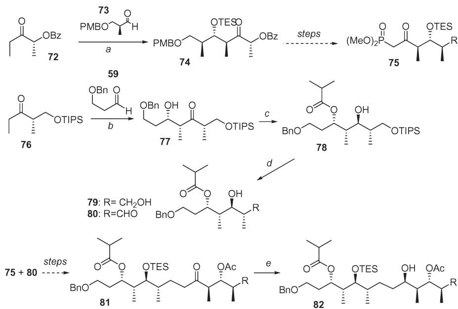
Scheme 9 a 1. (c-Hex) 2 BCl, Me 2 NEt, Et 2 O, 0 °C, 1 h, then –78 °C, 73 , to >–20 °C, 16 h; 2. TESOTf, 2,6-lutidine, CH 2 Cl 2 , –78 °C, 2 h; b Sn(OTf) 2 , Et 3 N, CH 2 Cl 2 , 59 , –78 °C, 2 h; c isobutyraldehyde, SmI 2 , THF, 0 °C, 2.5 h; d 1. HF·pyridine, THF, rt, 7 h; 2. cat. TEMPO, PhI(OAc) 2 , rt, 2 h; e SmI 2 , CH 3 CHO, THF, –5 °C, 2.5 h.
