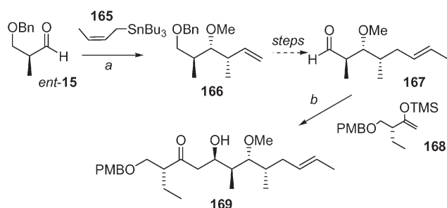
Scheme 21 a 1. 165, TiCl 4 2. KH, MeI; b 168, BF 3 ·OEt.
