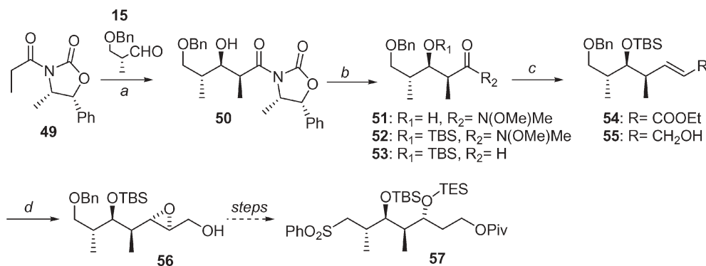
Scheme 6 a \text{Bu}_2\text{BOTf} , \text{Et}_3\text{N} , \text{CH}_2\text{Cl}_2 , 0\text{ }^{\circ}\text{C} , then 15 , -78\text{ }^{\circ}\text{C} , 3 h \rightarrow 0\text{ }^{\circ}\text{C} , 20 min; b 1. \text{Me}_3\text{Al} , \text{MeONHMe}\cdot\text{HCl} , THF, toluene, \text{CH}_2\text{Cl}_2 , -10 to >0\text{ }^{\circ}\text{C} , 1.6 h; 2. t\text{-BuMe}_2\text{SiOTf} , 2,6-lutidine, \text{CH}_2\text{Cl}_2 , 0\text{ }^{\circ}\text{C} , 1 h; 3. DIBAL-H, THF, hexane, -78\text{ }^{\circ}\text{C} , 2 h; c 1. (i\text{-PrO})_2\text{P(O)CH}_2\text{COOEt} , t\text{-BuOK} , THF, -78\text{ }^{\circ}\text{C} , 1 h to >0\text{ }^{\circ}\text{C} , 1.5 h; 2. DIBAL-H, \text{CH}_2\text{Cl}_2 , hexane, -78\text{ }^{\circ}\text{C} , 1 h; d \text{Ti(O-}i\text{-Pr)}_4 , (+)-DET, t\text{-BuOOH} , 4 Å MS, \text{CH}_2\text{Cl}_2 , -23\text{ }^{\circ}\text{C} , 1 h.
