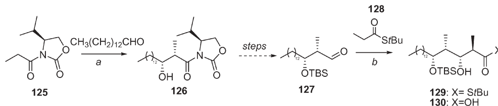
Scheme 15 a n -Bu 2 BOTf, Et 3 N, CH 2 Cl 2 , 0 °C, 0.5 h, then −78 °C, tetradecanal, 12 h; b 128 , (Chx) 2 BCl, Et 3 N, CH 2 Cl 2 , 0 °C, 2 h, then −78 °C, 127 , 12 h, oxidative work-up.
