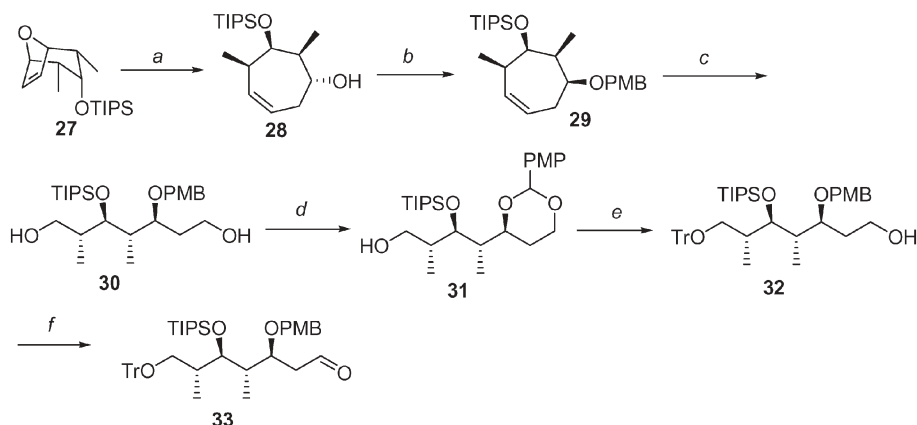
Scheme 3 a \text{Ni}(\text{COD})_2 , ( S )-BINAP, toluene, 65 °C, DIBAL-H (added over 20 h); b 1. DMSO, (\text{COCl})_2 , \text{NEt}_3 , \text{CH}_2\text{Cl}_2 , -78 °C; 2. toluene, DIBAL-H, -78 °C; 3. THF, KHMDS, PMBCl; c \text{O}_3 , \text{MeOH}/\text{CH}_2\text{Cl}_2 , -78 °C then \text{NaBH}_4 , rt; d \text{CH}_2\text{Cl}_2 , DDQ, mol. sieves; e 1. TrCl, \text{Et}_3\text{N} , DMAP, \text{CH}_2\text{Cl}_2 ; 2. \text{CH}_2\text{Cl}_2 , DIBAL-H, -78 °C - >0 °C; f DMSO, (\text{COCl})_2 , \text{NEt}_3 , \text{CH}_2\text{Cl}_2 , -78 °C.
