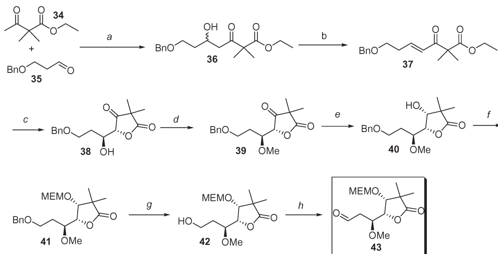
Scheme 4 a LDA, the ketone 34 , 1 h., then the aldehyde 35 , THF, -78 °C, 1 h; b \text{MsCl} , \text{NEt}_3 , \text{CH}_2\text{Cl}_2 0 °C, 4.5 h; c (\text{DHQD})_2\text{PYR} , \text{K}_3\text{Fe}(\text{CN})_6 , \text{K}_2\text{CO}_3 , \text{NaHCO}_3 , \text{MeSO}_2\text{NH}_2 , \text{OsO}_4 , \text{H}_2\text{O}/t\text{-BuOH} 0 °C, 17 h; d \text{MeI} , \text{Ag}_2\text{O} , \text{Et}_2\text{O} , reflux, 22 h; e LS-Selectride, THF, -78 °C, 15 min; f \text{MEMCl} , DIPEA, \text{CH}_2\text{Cl}_2 , reflux, 48 h; g \text{Pd}(\text{OH})_2/\text{C} , \text{EtOH} , \text{H}_2 , 40 min; h TPAP, \text{CH}_2\text{Cl}_2 , 4 Å MS, 2 h.
