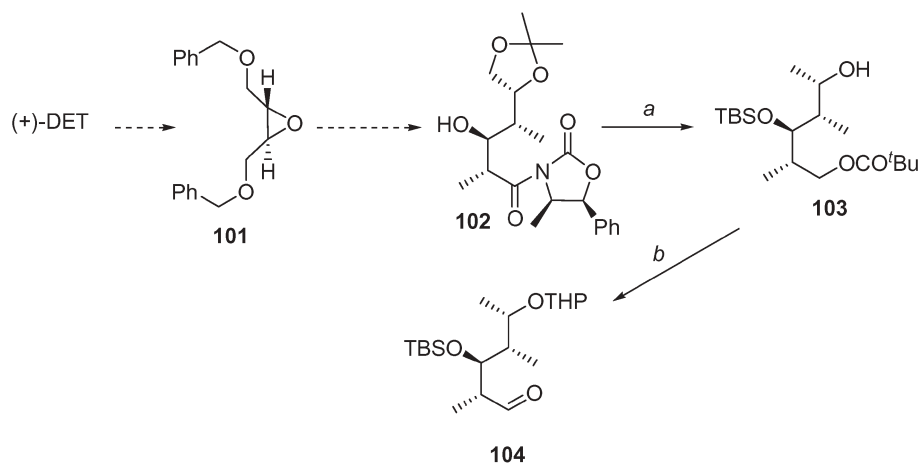
Scheme 12 a 1. \text{LiBH}_4 , THF, 0^\circ\text{C} , 0.5 h, then t\text{-BuCOCl} , pyridine, 3 h; 2. \text{Me}_2\text{-}t\text{-BuSiOTf} , 2,6-lutidine, \text{CH}_2\text{Cl}_2 , 0^\circ\text{C} , 1 h, then \text{AcOH} –THF– \text{H}_2\text{O} (3 : 1 : 1), 50^\circ\text{C} , 2 h; 3. \text{PhSSPh} , n\text{-Bu}_3\text{P} , THF, 0\text{--}25^\circ\text{C} , 3 h, then Raney Ni, EtOH, 12 h; b 1. dihydropyran, cat. CSA, \text{CH}_2\text{Cl}_2 , 0\text{--}25^\circ\text{C} , 3 h; 2. DIBAL-H, \text{CH}_2\text{Cl}_2 , -78^\circ\text{C} , 0.5 h, then \text{CrO}_3 , \text{HCl} –pyr, NaOAc, \text{CH}_2\text{Cl}_2 , 25^\circ\text{C} , 4 h.
